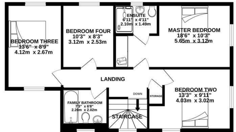
1ST FLOOR 652 sq.ft. (60.6 sq.m.) approx.
